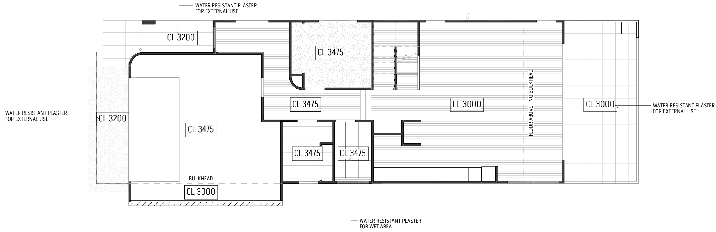
1 A-03-01/ GROUND FLOOR CEILING PLAN SCALE 1 : 100
