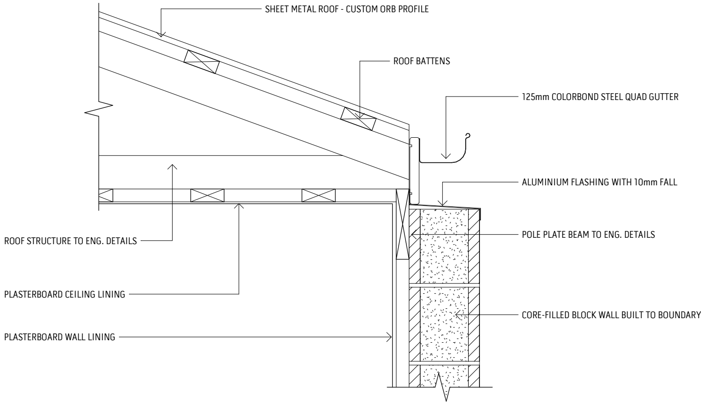
GUTTER OVER BLOCKWORK
