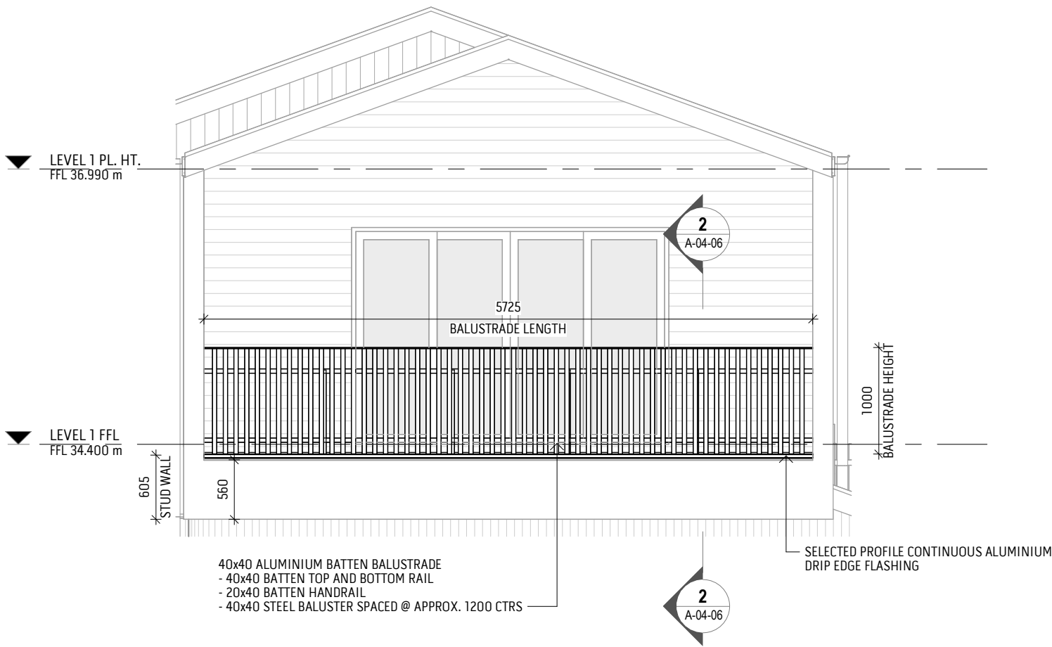
1 / BALUSTRADE DETAIL SCALE 1 : 50
