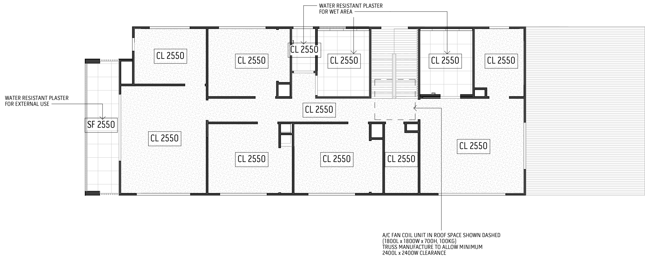
1 A-03-01 / LEVEL 1 CEILING PLAN SCALE 1 : 100
