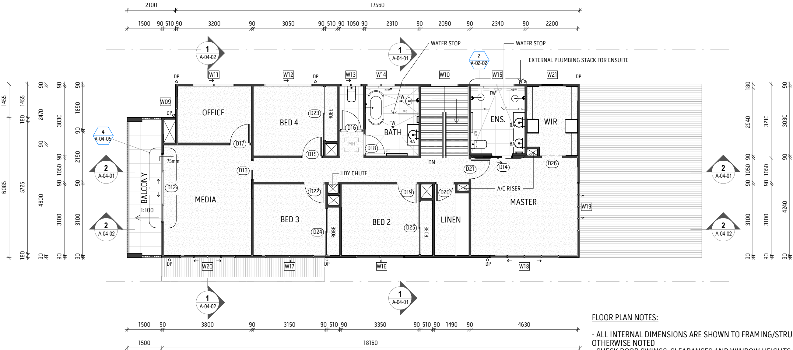
LEVEL 1 FLOOR PLAN
