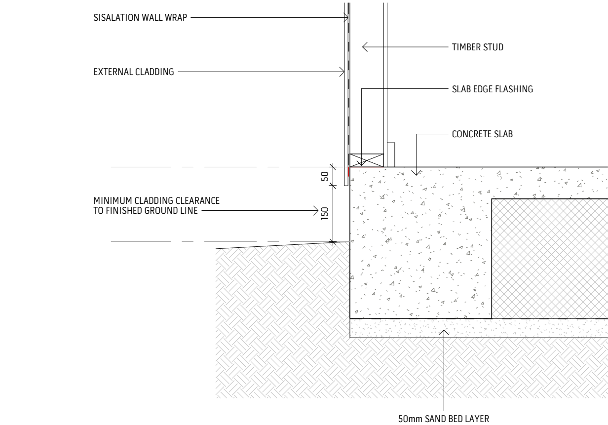
SLAB EDGE DETAIL - CLADDING
