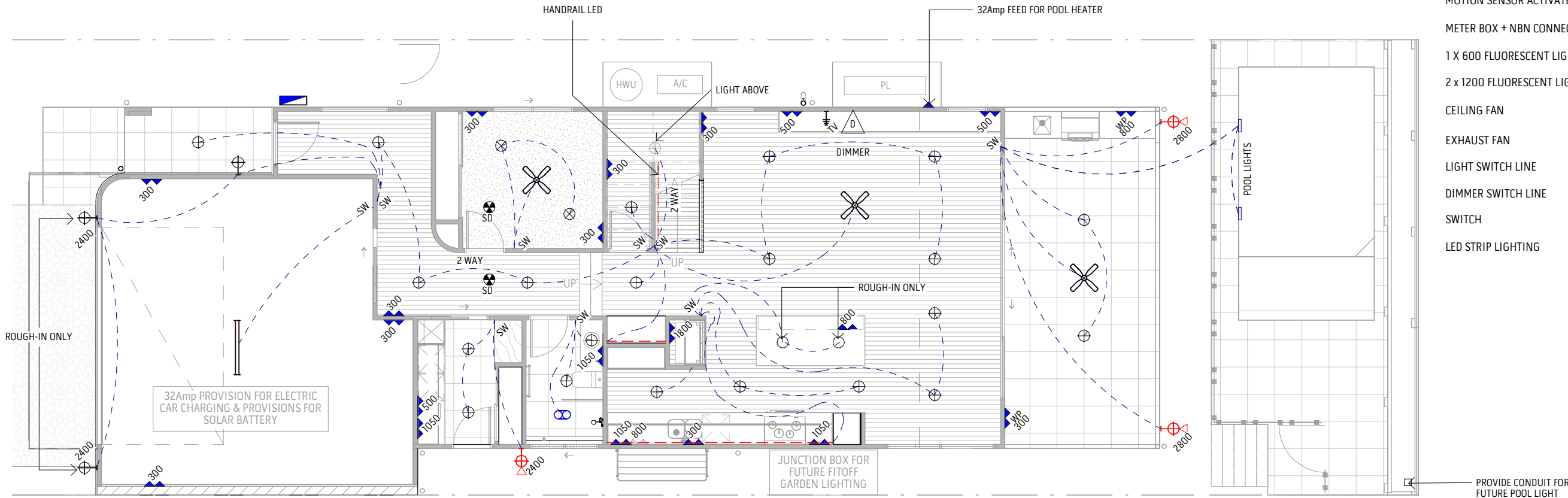
1 A-03-01 GROUND FLOOR ELECTRICAL PLAN SCALE 1 : 100
