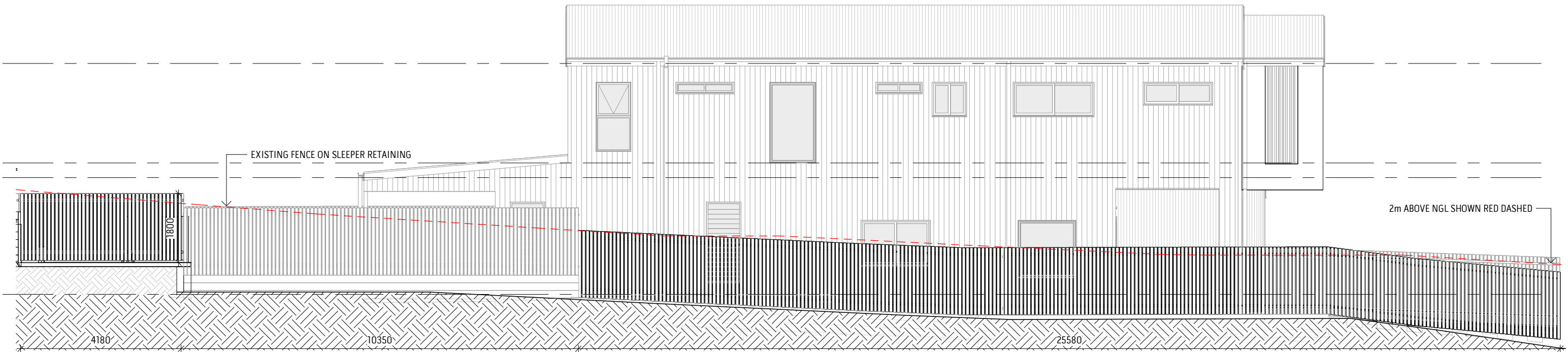
FENCE ELEVATION A
