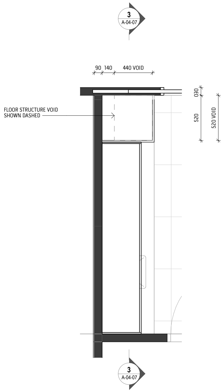
1 / A-03-01 / LAUNDRY CHUTE GROUND SCALE 1 : 25
