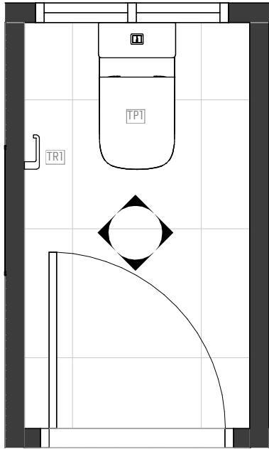
1 A-03-01/ INTERNAL - UPPER TOILET SCALE 1 : 25
