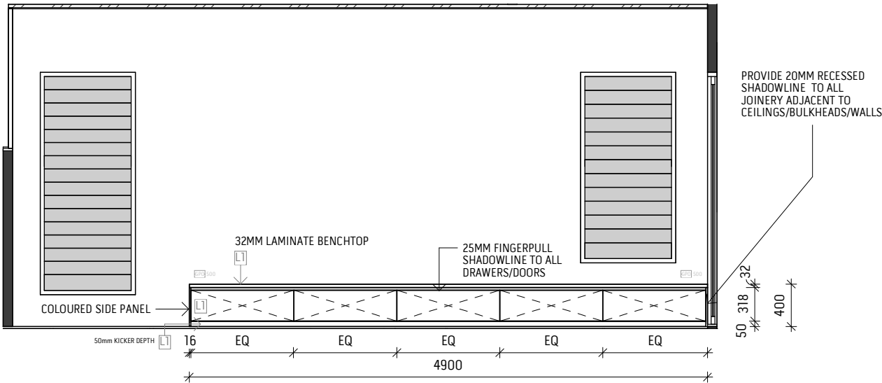
2 TV CABINET SECTION SCALE 1 : 50
