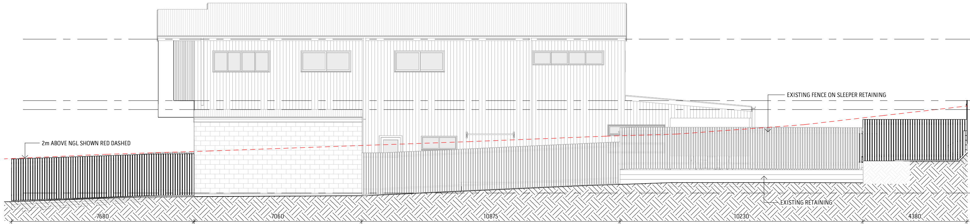
FENCE ELEVATION B
