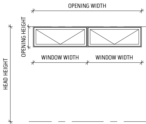
AWNING - AA
